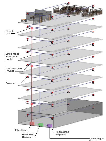
TYPICAL DAS DIAGRAM
